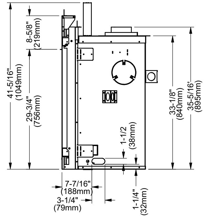
SIDE VIEW
